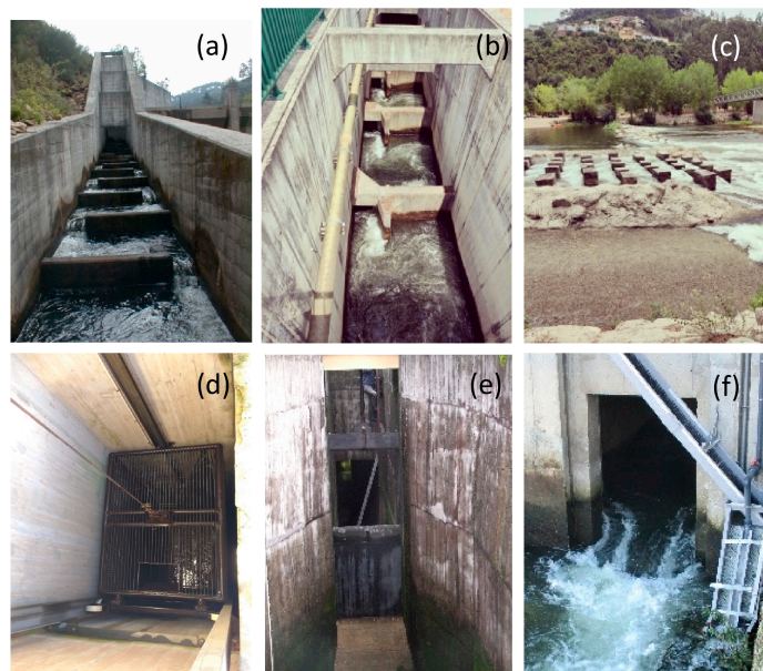
Figure 1. Most common types of fishways addressed in the present study: (a) PaW at São Pedro do Sul (#53); (b) VSF at Ponte de Coimbra I (#78); (c) nature-like (fish ramp) at Palheiros (#76); (d) fish lift at Touvedo (#8); (e) fish lock at Crestuma-Lever (#37) and (f) eel pass at Ponte de Coimbra II (#77). Combined systems (e.g., PaW with fish lift) are also present (fishways codes are provided in Table S1).
