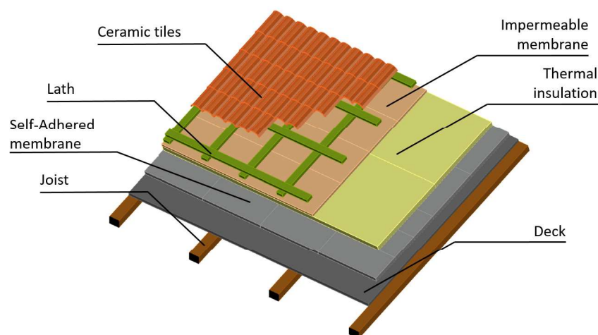
Figure 1. Description of roof layers in southern Europe.
