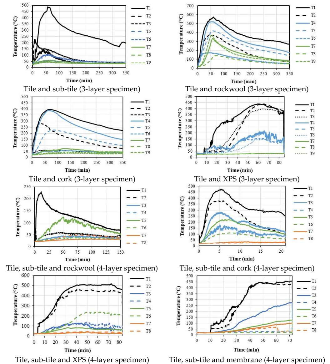
Figure 4. Temperature evolution measured at each layer for all roof specimens tested during exposure to firebrand accumulation.
