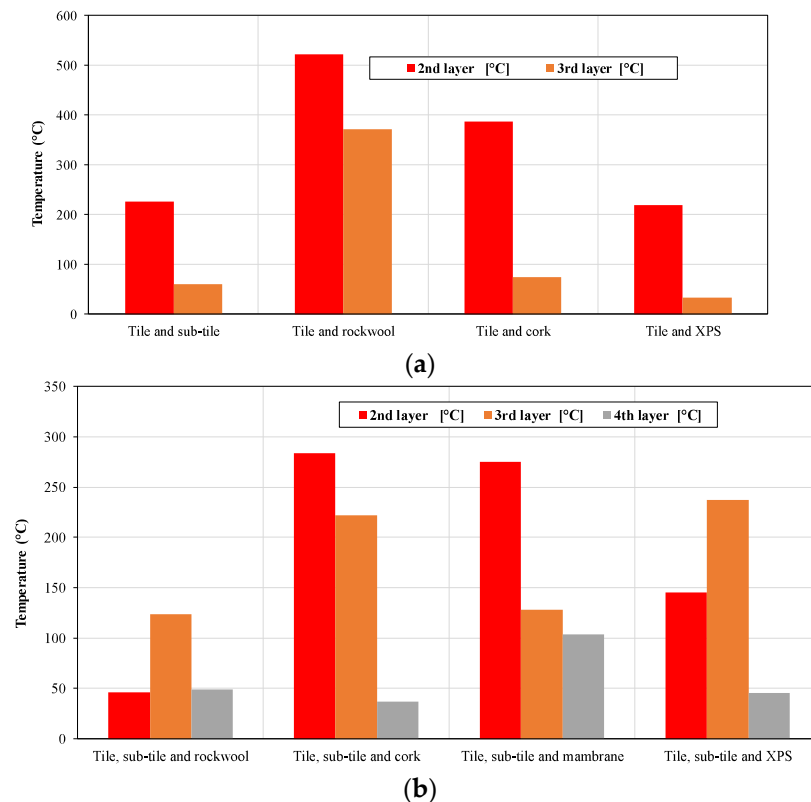
Figure 7. Maximum temperatures recorded in the 2nd, 3rd, and 4th layers for (a) three-layer specimens and (b) four-layer specimens.
