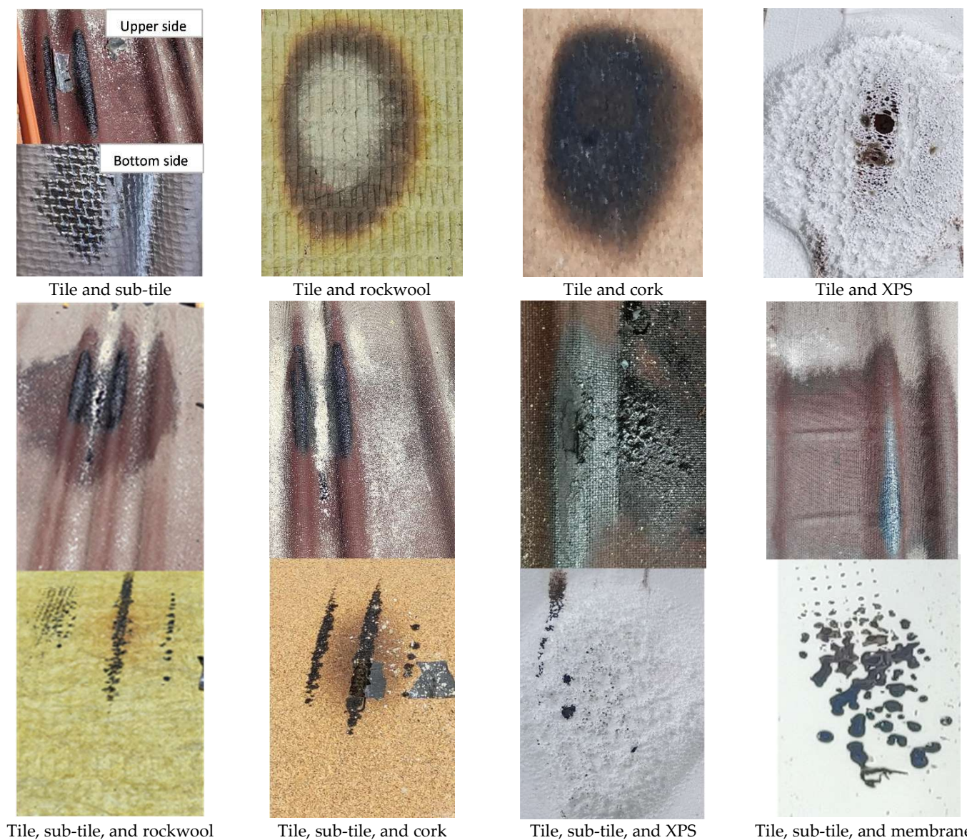
Figure 10. Impact of firebrand accumulation penetration in construction materials for each tasted specimen.
