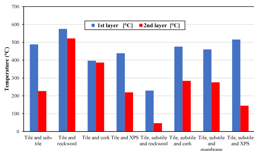
Figure 6. Maximum temperatures recorded in the 1st layer and 2nd layer for all roof specimens.
