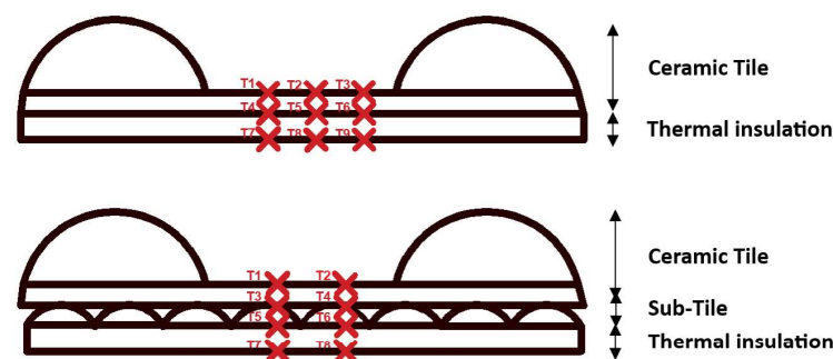
Figure 5. Position and numbering of the thermocouples for 3 and 4 layers.
