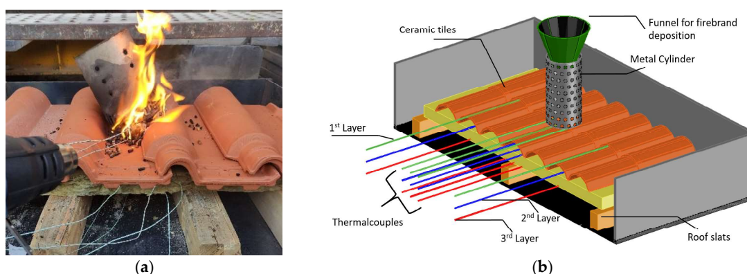
Figure 3. Test setup for firebrand accumulation in construction elements specimens with 3 layers. (a) Roof firebrand accumulation test. (b) Representation of thermocouple location in the roof specimens.
