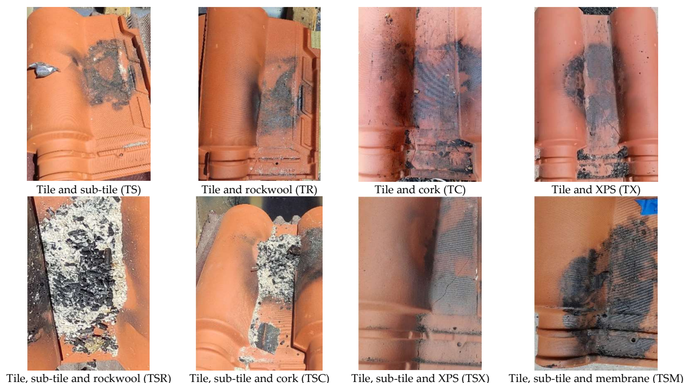
Figure 8. Tile condition of each specimen after exposure to firebrand accumulation test.
