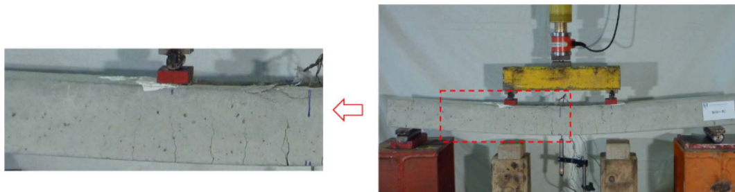
Fig. 13. Experimental cracks of four-point bending RC beam (Firmo 2015).
