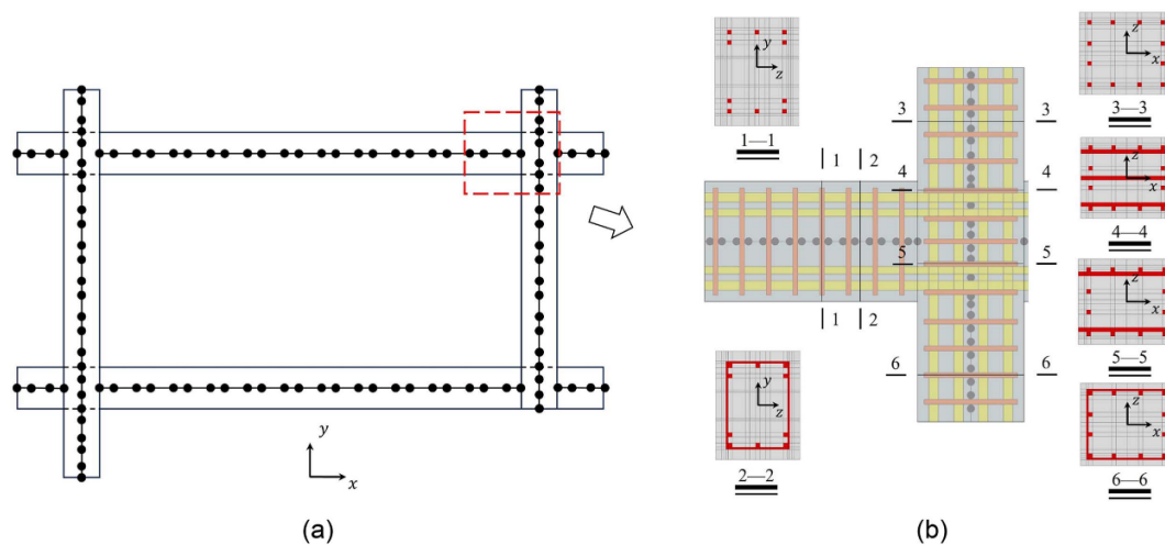
Fig. 23. (a) FE discretization of beam elements; and (b) cross-sectional discretization for the RC frame.
