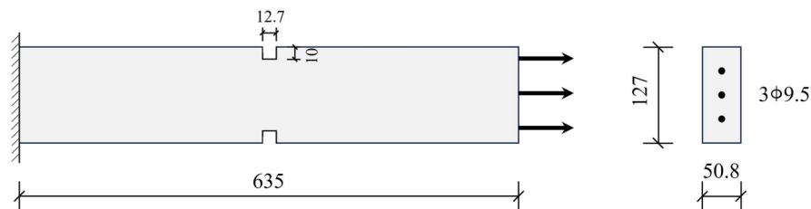
Fig. 3. Load layout and geometry of notched RC beams under direct tension (unit: mm).
