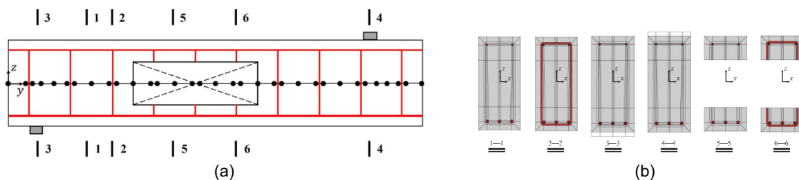
Fig. 17. (a) FE discretization of beam elements; and (b) cross-sectional discretization for the RC beam with web openings.
