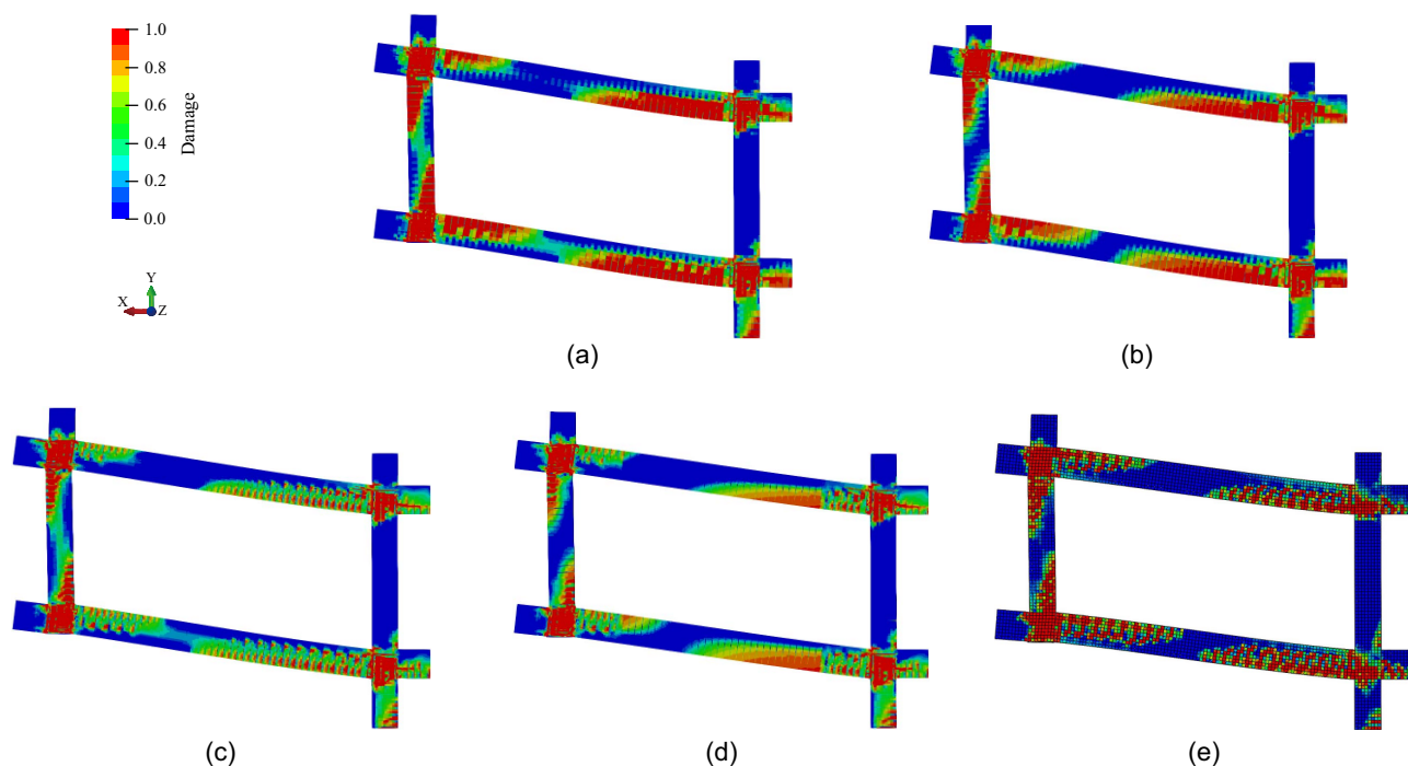
Fig. 26. Damage distributions of the RC frame from: (a) Model 1 (refined CW + B2); (b) Model 2 (NDK TE1 + B2); (c) Model 3 (refined CW + B3); (d) Model 4 (NDK TE1 + B3); and (e) ABAQUS model at the displacement of 140 mm (scale factor is 5).
