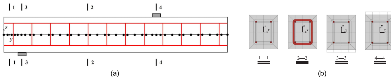
Fig. 9. (a) FE discretization of beam elements; and (b) cross-sectional discretization for the four-point bending RC beam.
