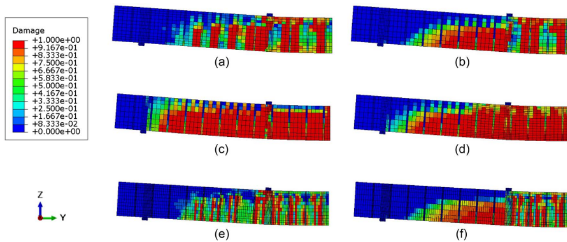
Fig. 12. Final damage distribution of four-point bending RC beams from: (a) Model 1 (refined CW + 40B2); (b) Model 2 (NDK1 + 40B2); (c) Model 3 (NDK2 + 40B2); (d) Model 4 (NDK3 + 40B2); (e) Model 5 (Refined CW + 40B4); and (f) Model 6 (NDK1 + 40B4).
