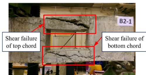
Fig. 20. Failures observed from experiments (Elsanadedy et al. 2019).
