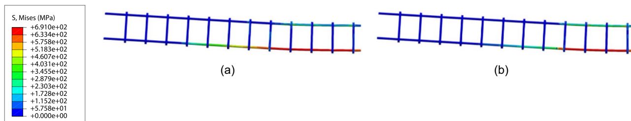
Fig. 15. Von Mises stress distribution of steel reinforcement in four-point bending RC beam from: (a) Model 5 (refined CW + 40B4); and (b) Model 6 (NDK1 + 40B4) at displacement of 25 mm.
