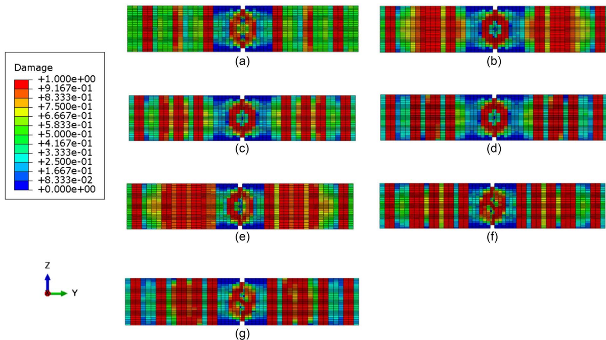
Fig. 7. Final damage distributions of the notched RC beam from: (a) Model 1 (refined CW); (b) Model 2 (NDK1 TE1); (c) Model 3 (NDK1 TE2); (d) Model 4 (NDK1 TE3); (e) Model 5 (NDK2 TE1); (f) Model 6 (NDK2 TE2); and (g) Model 7 (NDK2 TE3).
