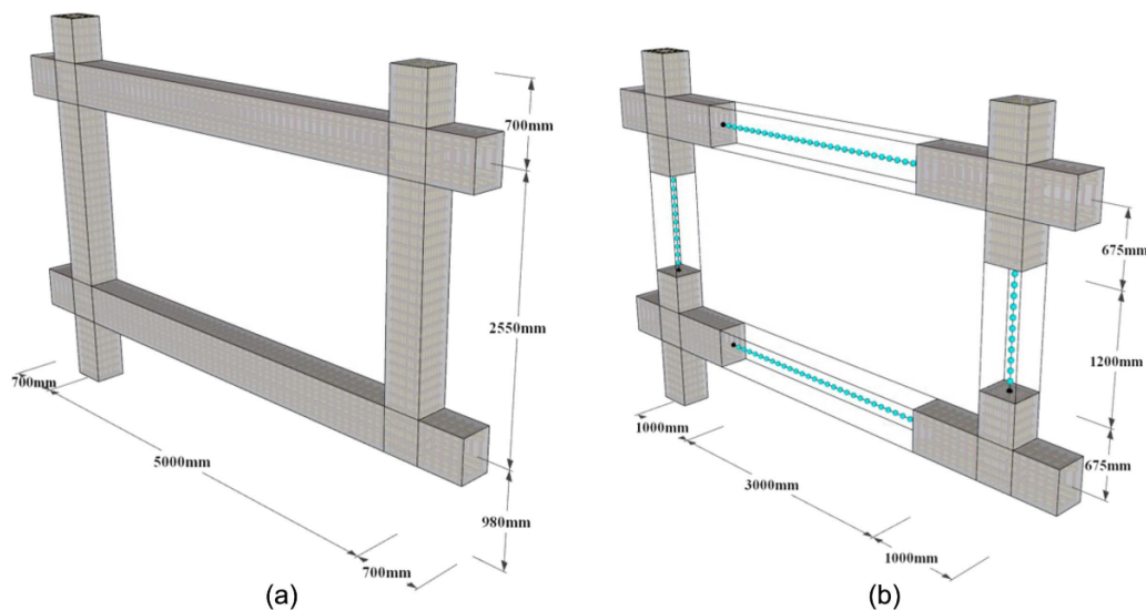
Fig. 24. (a) Refined CW model; and (b) NDK model for the analysis of the RC frame.
