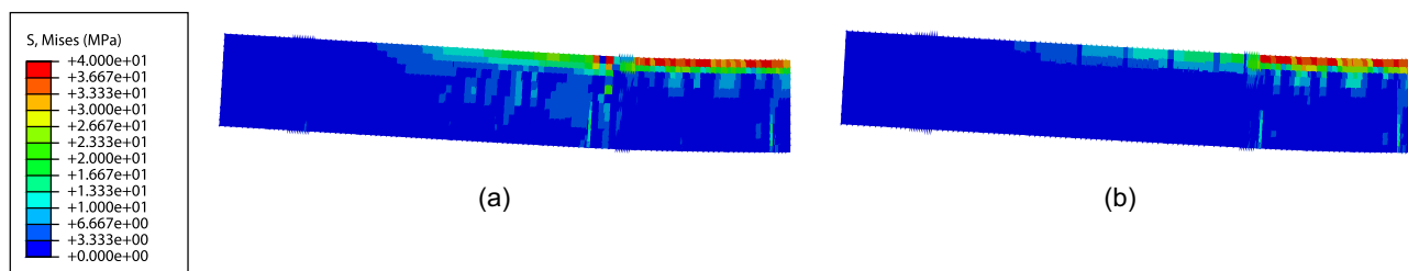
Fig. 14. Von Mises stress distribution of concrete in four-point bending RC beam from: (a) Model 5 (refined CW + 40B4); and (b) Model 6 (NDK1 + 40B4) at displacement of 25 mm.
