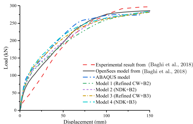
Fig. 25. Load–displacement curves for the RC frame.
