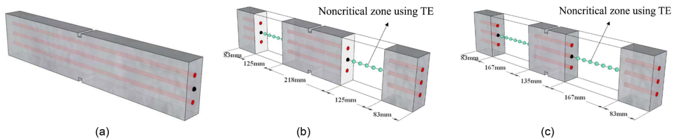
Fig. 5. Different models adopted for the analysis of the notched RC beam: (a) refined CW model; (b) NDK1 model; and (c) NDK2 model.
