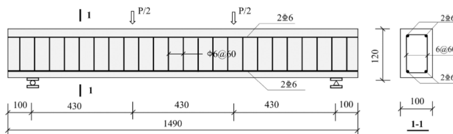
Fig. 8. Load layout and geometry of RC beams under four-point bending (unit: mm).
