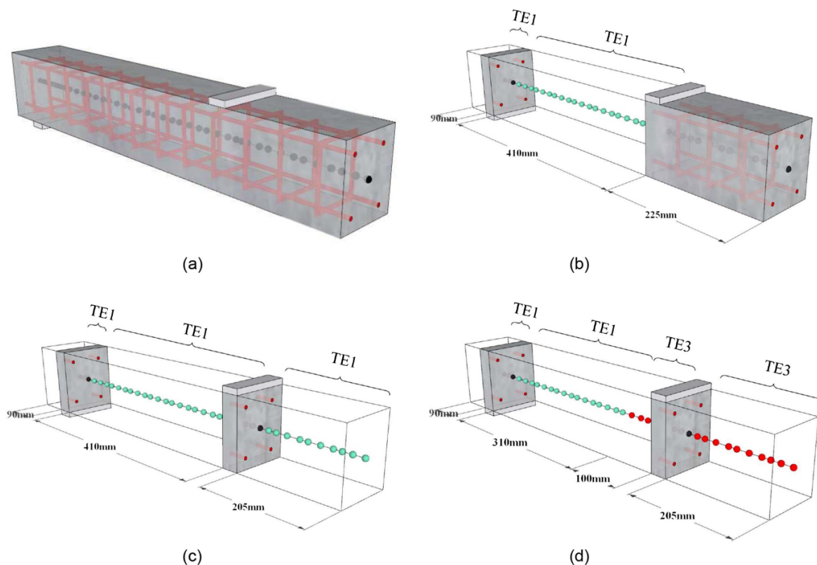
Fig. 10. Different models adopted for the analysis of the four-point bending RC beam: (a) refined CW model; (b) NDK1; (c) NDK2; and (d) NDK3.
