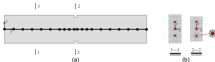
Fig. 4. (a) FE discretization of beam elements; and (b) cross-sectional discretization for the notched RC beam.
