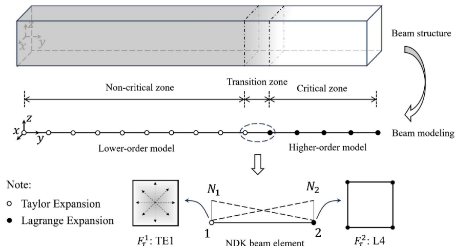
Fig. 2. A CUF-based 1D model with NDK approach.
