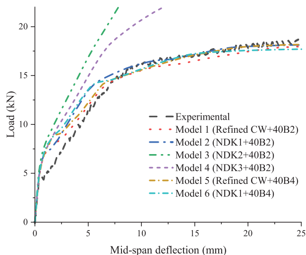
Fig. 11. Load-deflection curves for four-point bending RC beams.
