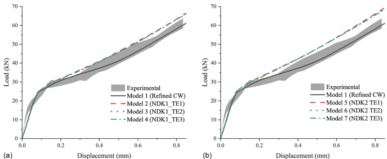
Fig. 6. Load–deflection curves from experimental test, refined CW model: (a) NDK1 models; and (b) NDK2 models for the notched RC beam.
