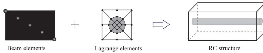
Fig. 1. An illustration of the beam model with CW approach for modeling RC structures.
