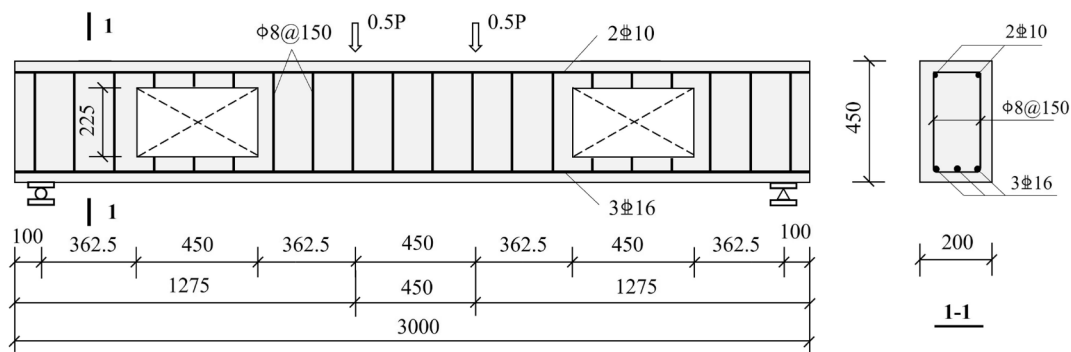
Fig. 16. Load layout and geometry of the RC beam with web openings (unit: mm).
