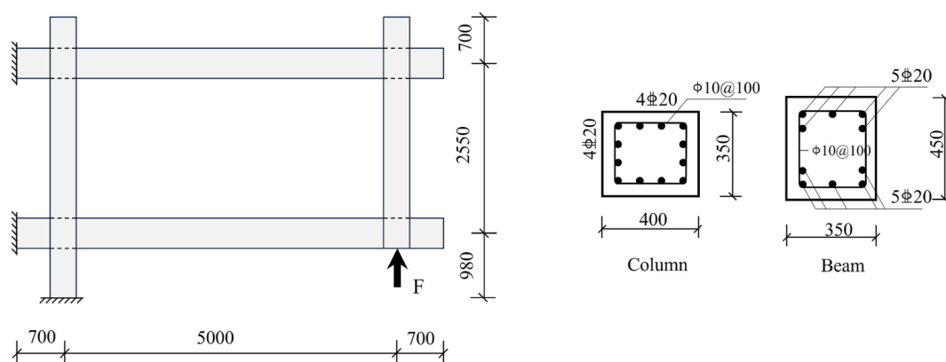
Fig. 22. Load layout and geometry of the studied RC frame (unit: mm).
