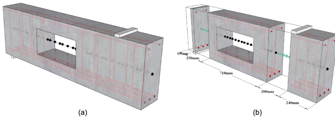
Fig. 18. (a) Refined CW model; and (b) NDK model for the analysis of the RC beam with web openings.
