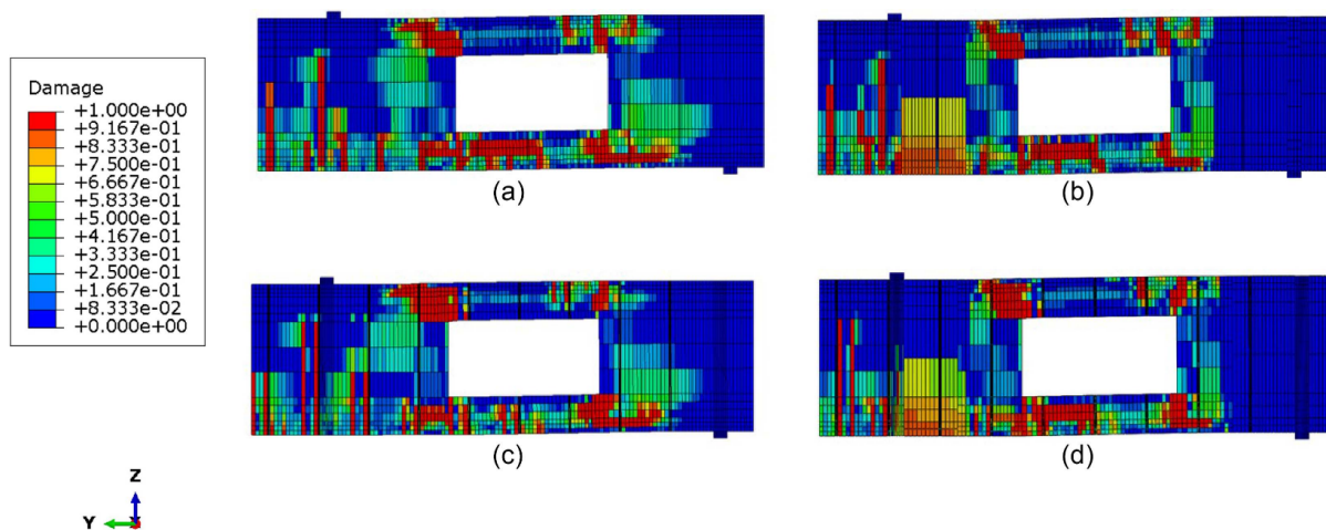
Fig. 21. Damage distributions of the RC beam with web openings from: (a) Model 1 (refined CW + 79B2); (b) Model 2 (NDK + 79B2); (c) Model 3 (refined CW + 42B4); and (d) Model 4 (NDK + 42B4) at the displacement of 11 mm.
