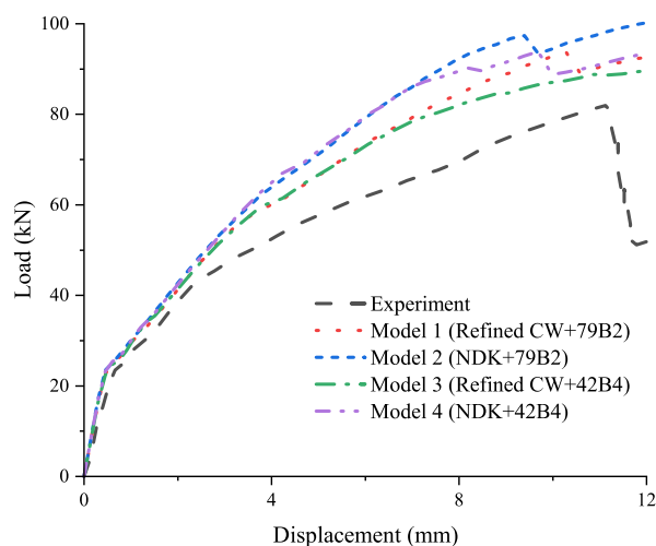
Fig. 19. Load-displacement curves for RC beam with web openings.
