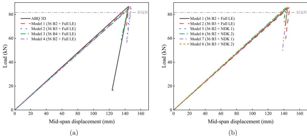
Fig. 21. Load-displacement (mid-span) curves of the FPB beam from various numerical models.
