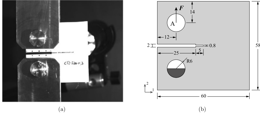
Fig. 5. (a) Experimental layout [54] and (b) geometry for CT test (mm).
