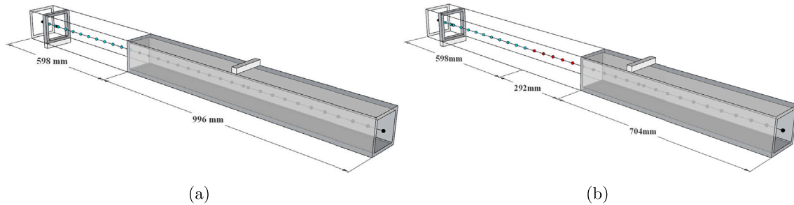
Fig. 20. (a) NDK 1 model and (b) NDK 2 model for the FPB beam—Black represents LE, cyan stands for TE1, and red denotes TE3.
