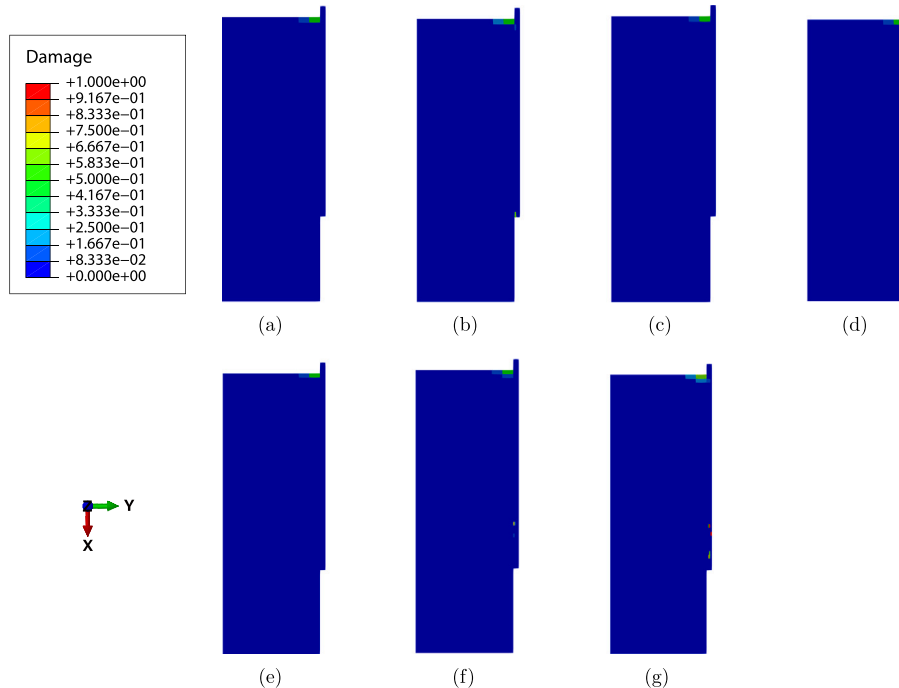
Fig. 13. Matrix compressive damage distribution of the TPB beam from (a) Model 1; (b) Model 2; (c) Model 3; (d) Model 4; (e) Model 5; (f) Model 6; (g) Model 7.
