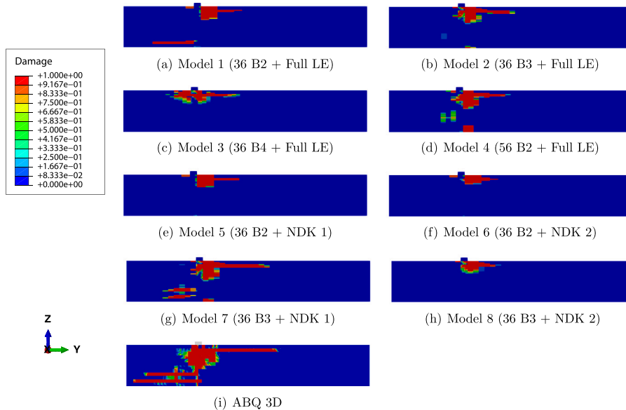
Fig. 25. Shear damage distribution of the FPB beam from various models.
