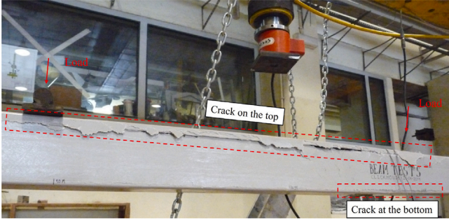
Fig. 24. Experimental failure mode of the FPB beam [57].
