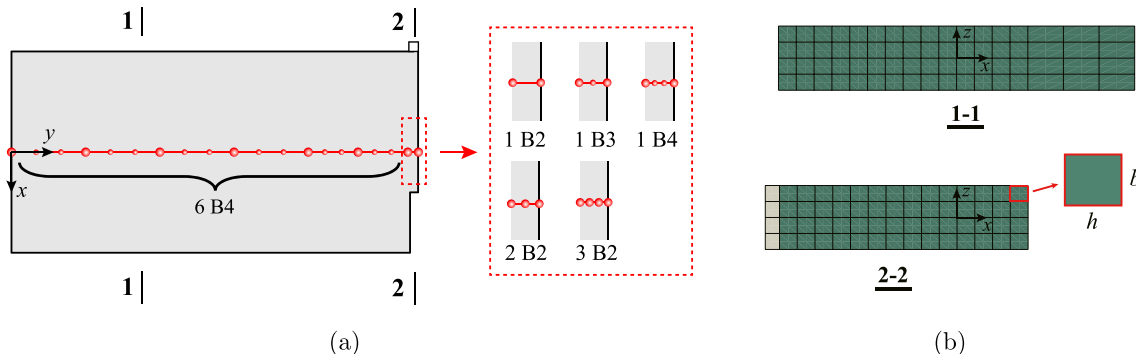
Fig. 10. (a) Beam element and (b) cross-sectional discretizations of the TPB beam.
