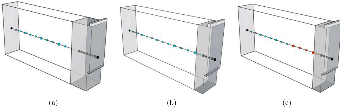
Fig. 14. (a) NDK 1 model, (b) NDK 2 model, and (c) NDK 3 model based on Model 1 for the analysis of the TPB beam-Cyan represents TE1 and red denotes TE3.
