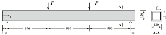
Fig. 18. Loads and geometry of the FPB beam (mm).
