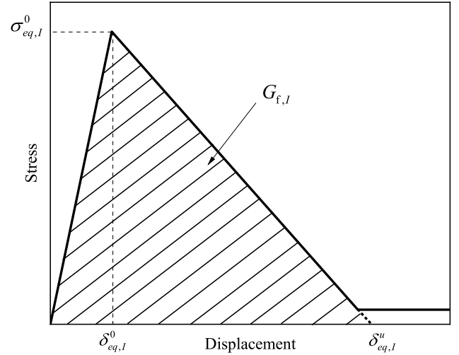
Fig. 3. Equivalent displacement-stress for fiber, matrix, and interlaminar.
