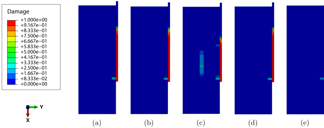
Fig. 16. Matrix tensile damage distribution of the TPB beam from (a) Model 8; (b) Model 9; (c) Model 10; (d) Model 11; (e) Model 12.
