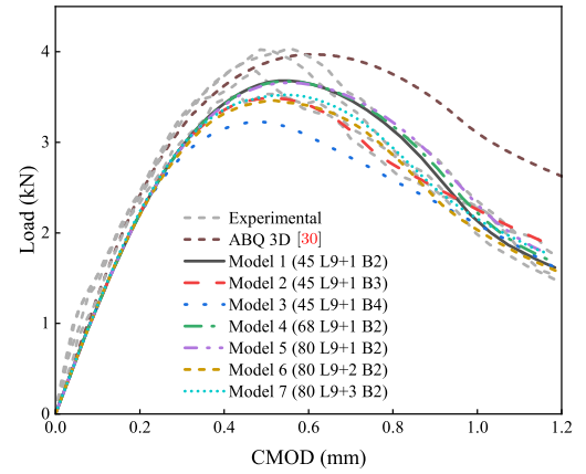
Fig. 11. Load-CMOD curves of the TPB beam across different CUF models.
