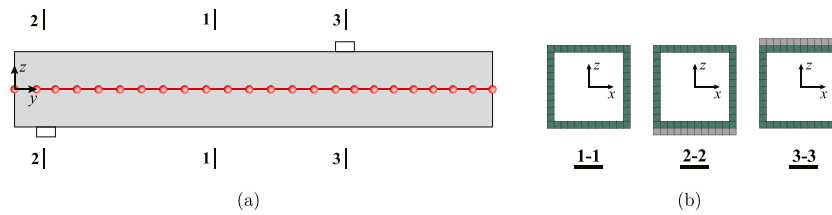
Fig. 19. (a) Beam element and (b) cross-sectional discretizations of the FPB beam.
