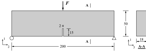
Fig. 9. Load and geometry of the TPB beam (mm).
