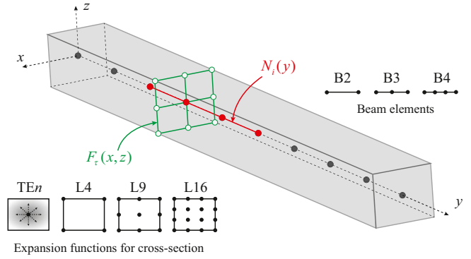
Fig. 1. Reference framework, beam elements, and cross-section expansion.
