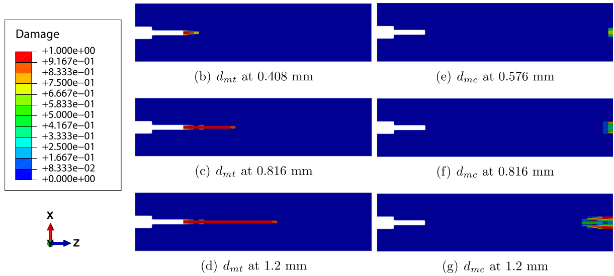
Fig. 8. Tensile and compressive matrix damage propagations of the CT test from Model 5.
