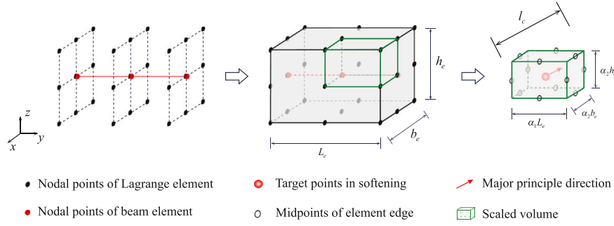
Fig. 4. Illustration of calculation for l_c .
