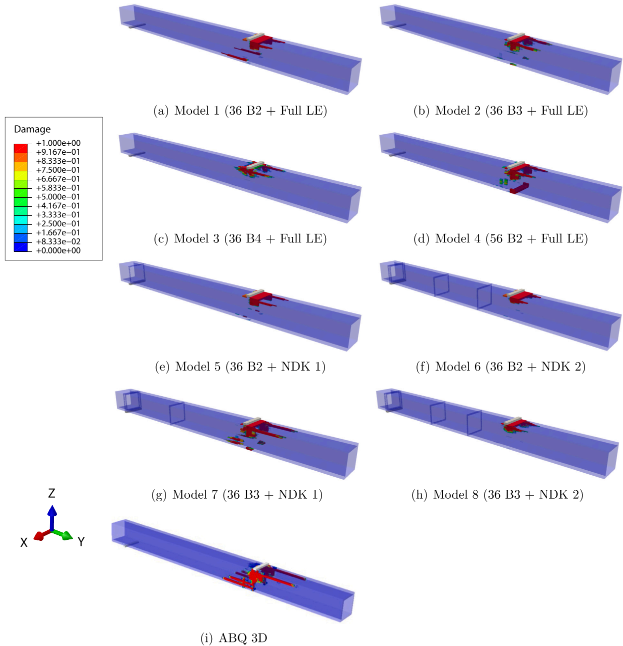
Fig. 26. 3D shear damage distribution of the FPB specimen.
