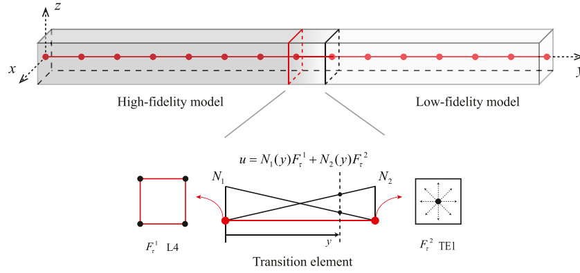
Fig. 2. NDK approach for CUF-based beam models.
