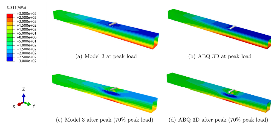
Fig. 22. Comparison of stress distribution \sigma_{11} between CUF and ABQ 3D models.
