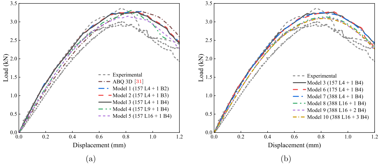
Fig. 7. Reaction load-displacement curves of the CT test from various CUF-based models: (a) Influence of order and (b) influence of mesh size.
