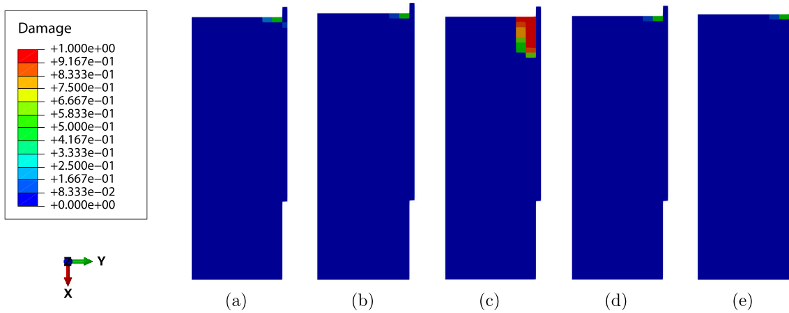
Fig. 17. Matrix compressive damage distribution of the TPB beam from (a) Model 8; (b) Model 9; (c) Model 10; (d) Model 11; (e) Model 12.
