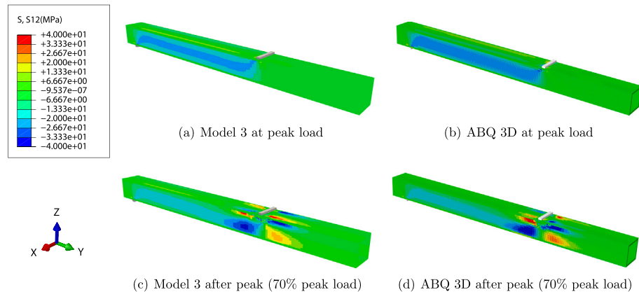
Fig. 23. Comparison of stress distribution \sigma_{12} between CUF and ABQ 3D models.
