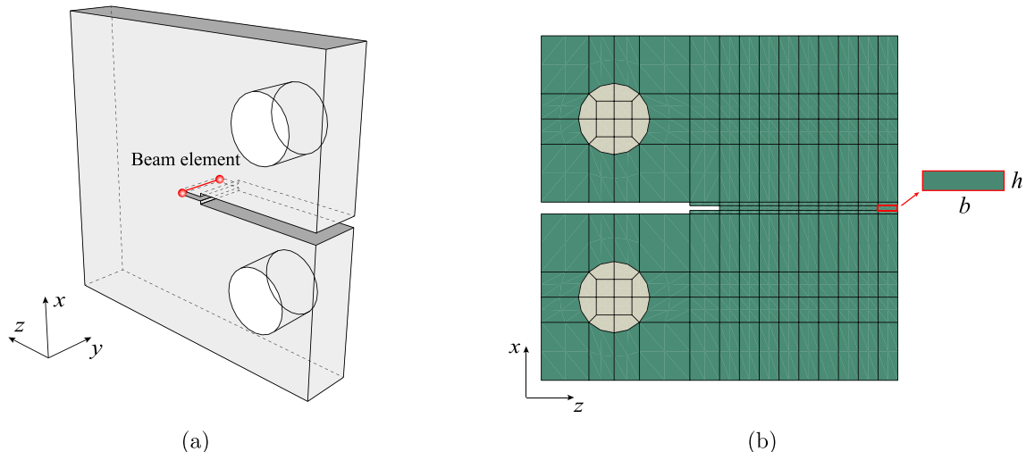
Fig. 6. (a) Beam elements and (b) cross-sectional discretizations of the CT specimen.
