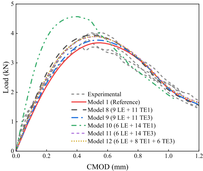
Fig. 15. Load-CMOD curves of different NDK models for the TPB beam.
